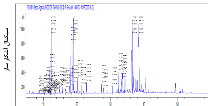
Figure (5): Gas chromatogram of Pulicaria gnaphalodes essential oil in Darab city (Konarhagi region)
