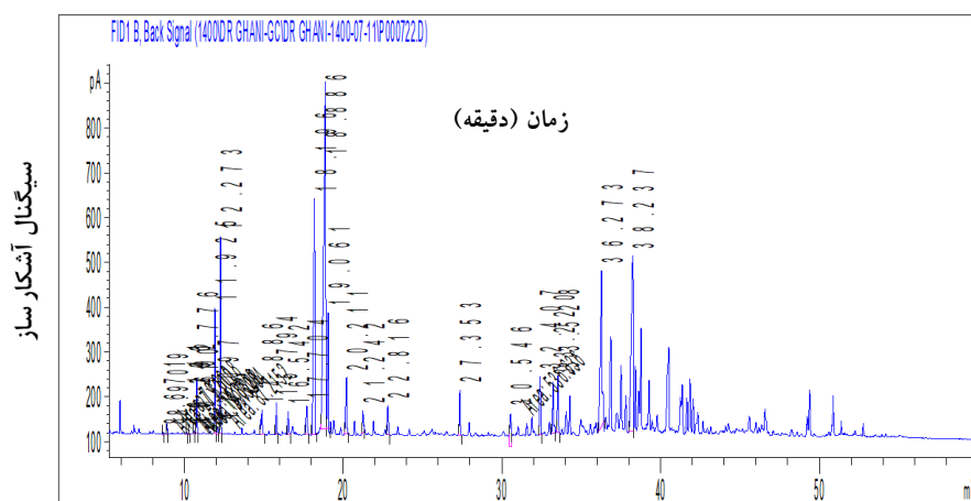
Figure (9): Gas chromatogram of Pulicaria gnaphalodes essential oil in Darab city (Tangeh Raghz region)
