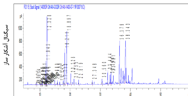
Figure (6): Gas chromatogram of Pulicaria gnaphalodes essential oil in Darab city (Jannt Shahr region)
