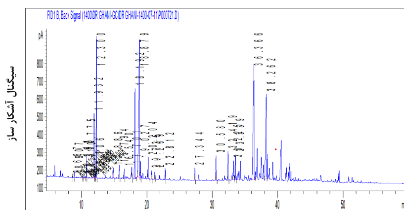
Figure (8): gas chromatogram of Pulicaria gnaphalodes essential oil in Darab city (Tang Katouye region)
