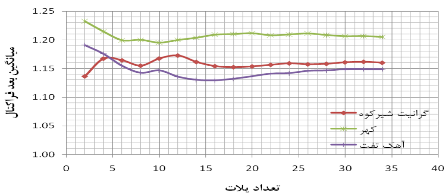
Figure (4): Fractal dimension changes with the number of selected plots from each geological formation
